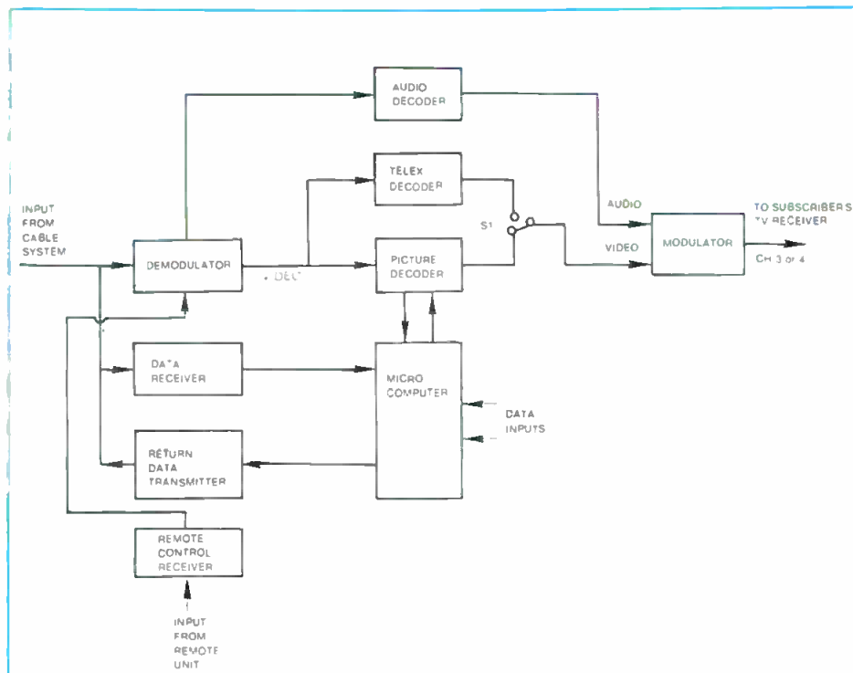
Figure 2. Future subscriber terminal.
