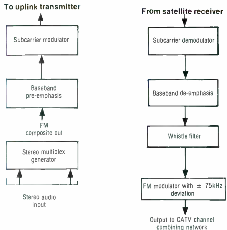
Figure 2. The Leaming composite subcarrier stereo transmission system.
