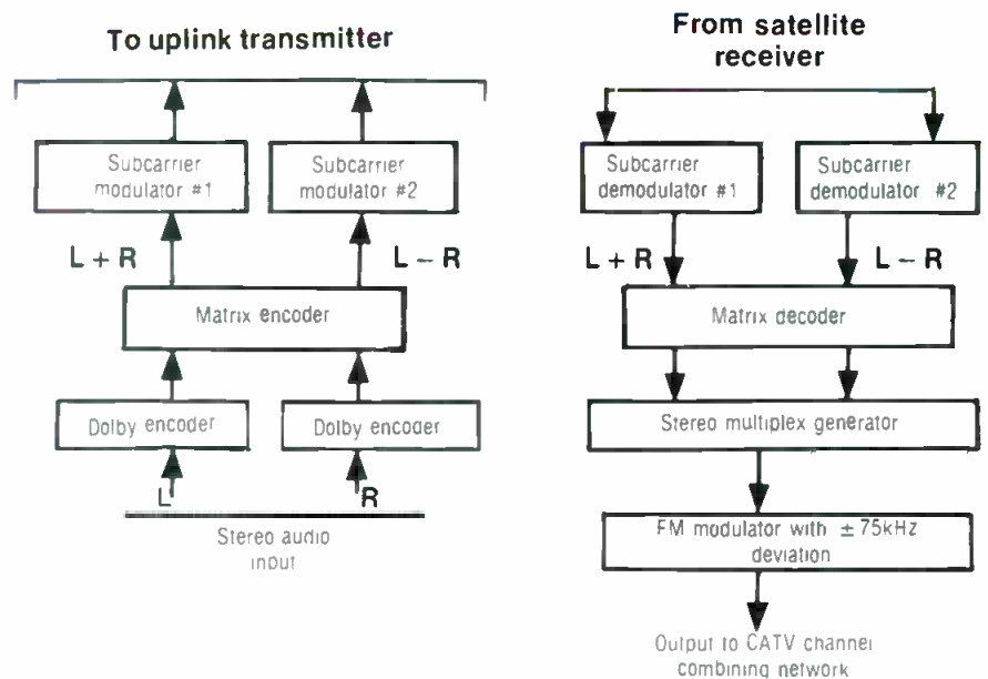
Figure 1. The Warner Amex stereo transmission system.
